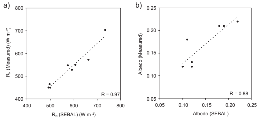
Fig. 4. Correlations between the estimated values by the SEBAL algorithm and measured values of R_N (a) and surface albedo (b) at the study area.
