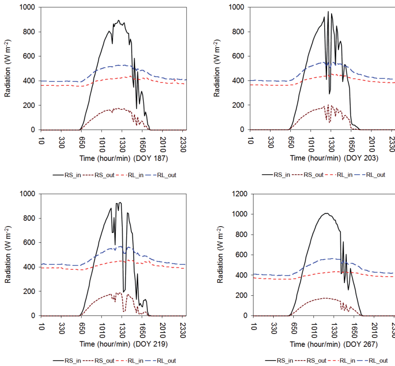
Fig. 2. Diurnal behavior of the incoming and outgoing shortwave (RS_in and RS_out) and longwave (RL_in and RL_out) radiation for different dates at the pasture site (FNS).
