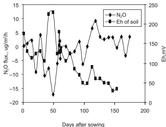
Fig. 4. Variation in N_2O flux in Vigna radiata field (Raghunathpur 2005) with redox potential during Rabi season.
