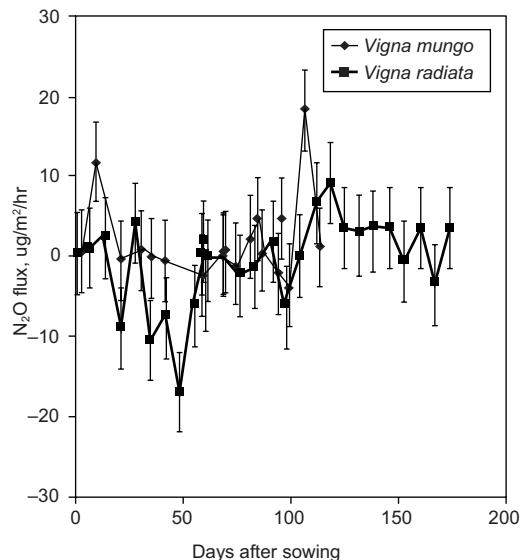
Fig. 2. Emissions of \text{N}_2\text{O} from Vigna mungo and Vigna radiata during the cropping season.
