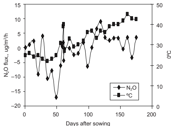
Fig. 5. Variation of N_2O flux with soil temperature in Vigna radiata field (Raghunathpur 2005) during Rabi season.
