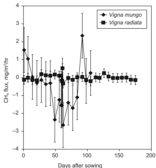
Fig. 1. Emission of \text{CH}_4 from Vigna mungo and Vigna radiata fields during the cropping season.
