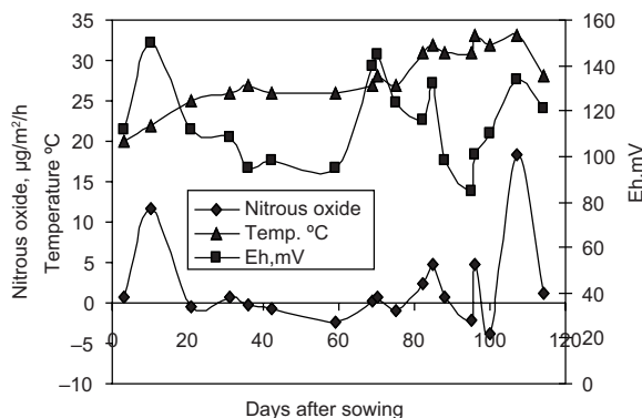
Fig. 3. Variation of \text{N}_2\text{O} flux with temperature and redox potential for Vigna mungo during Rabi season (Ragunathpur).
