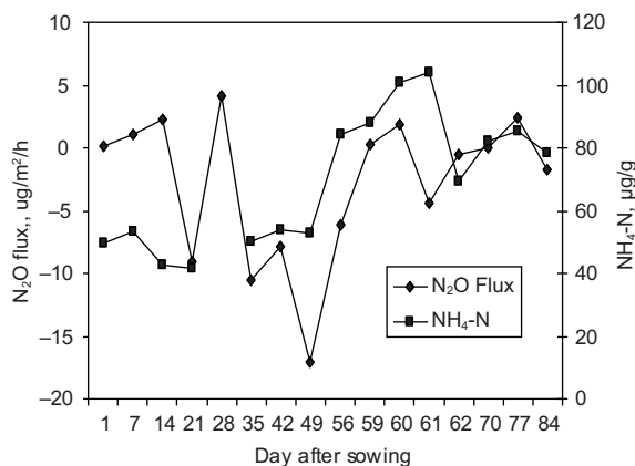
Fig. 6. Variation of N 2 O with NH 4 -N.
