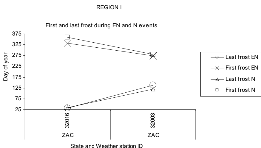
Fig. 3. Early and late frost dates for FFP during EN and N years in region I.
